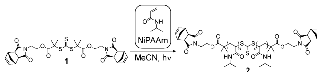
Scheme 1. Bis-norbornene TTC ( 1 ) used for the photo-controlled radical polymerization (photo-CRP) of NiPAAm.
